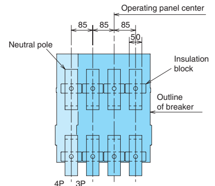
Front terminal
