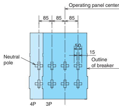
Vertical terminal
