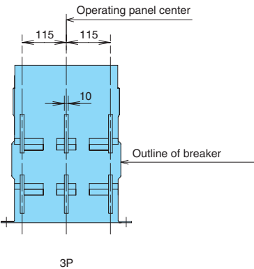
Main circuit terminal dimension
