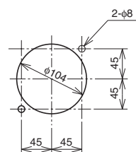
Drilling plan
