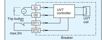
UVT circuit diagram (In case of 380-460V AC)
