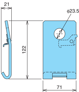
Lifting hooks (HP)
